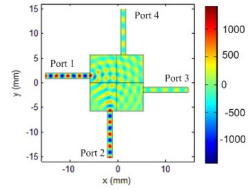
Fig. 4. The electric field distribution of beam shifter and normal slab
